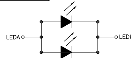
CONSTANT CURRENT:45mA,3.2V(REF.) BACKLIGHT DRIVER CIRCUIT DIAGRAM
